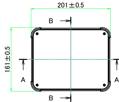
E view
